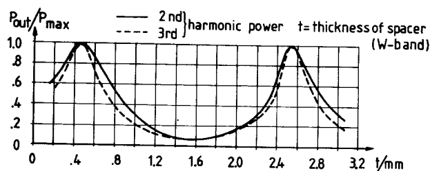
Fig. 3 Influence of the idler circuit
